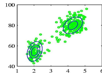
Mixture of 2 Gaussians
