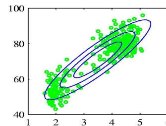
Single Gaussians
